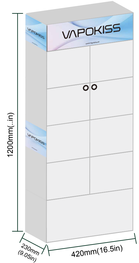
Acrylic Showcase
