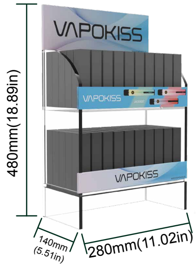
Acrylic Display
